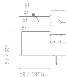
LOW FITTED-OUT ARM (OPTIONAL BOX)
