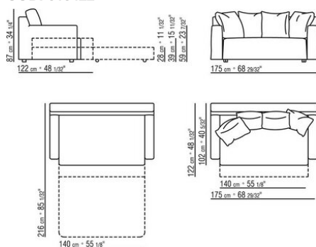
COD. 010422 WINNYQUATTRO SOFA/SINGLE BED
