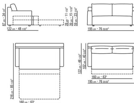
COD. 010413 SOFA/DOUBLE BED
