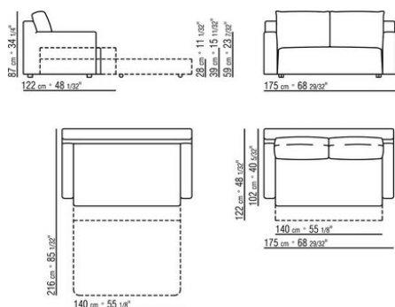
COD. 010412 SOFA/SINGLE BED
