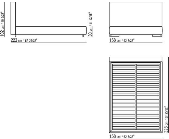
COD. 011UN6 QUEEN SIZE BED W/STORAGE
