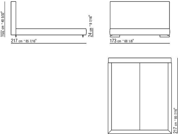
COD. 011UL2 BED WOODEN BASE
