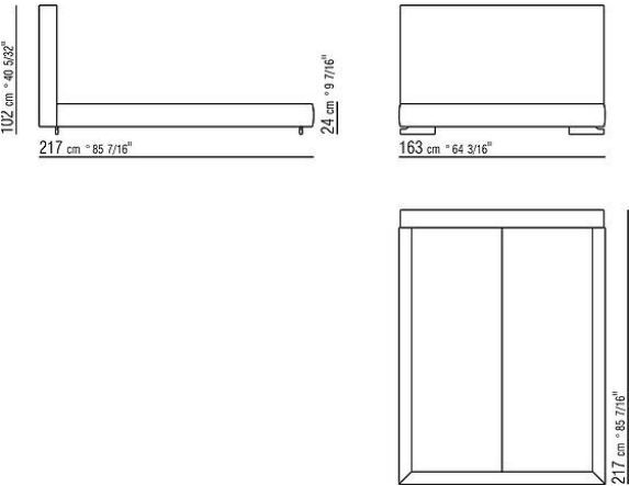
COD. 011UL1 BED WOODEN BASE
