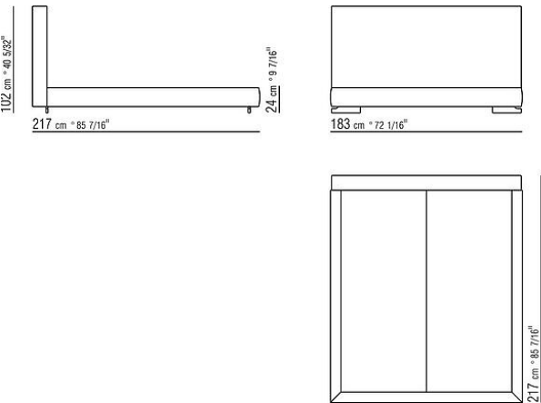
COD. 011UL3 BED WOODEN BASE
