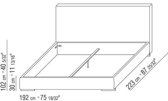
COD. 011UVC BED WITHOUT PLATFORM
