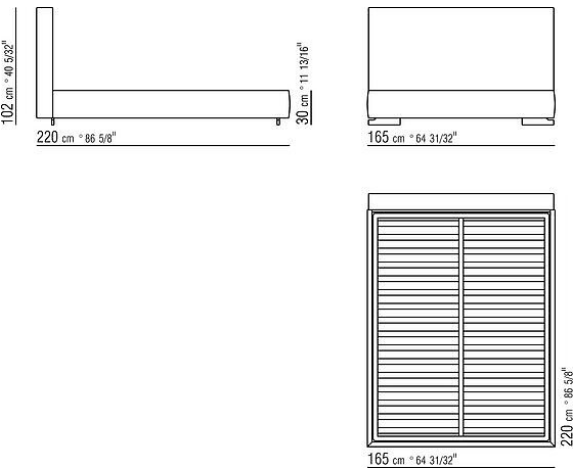
COD. 011UN1 BED W/STORAGE
