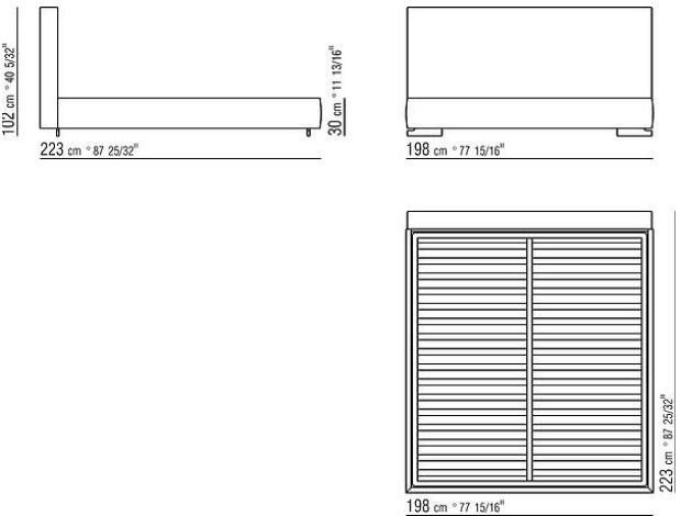
COD. 011UN8 KING SIZE BED W/STORAGE
