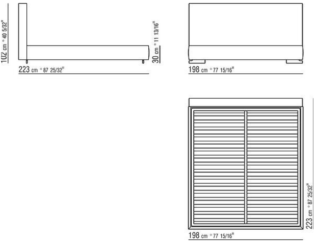
COD. 011UM8 KING SIZE BED W/ SLATS
