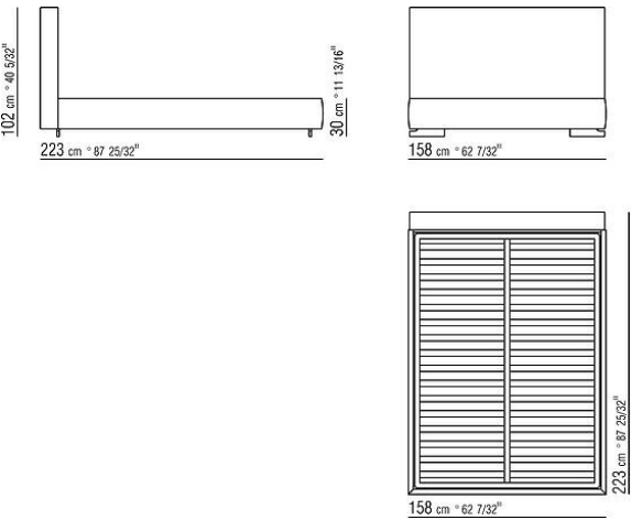
COD. 011UM6 QUEEN SIZE BED W/ SLATS
