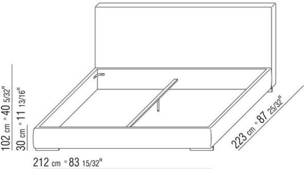
COD. 011UVE BED WITHOUT PLATFORM
