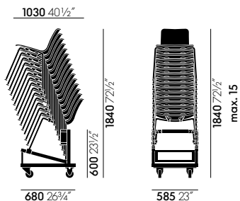
HAL Tube Stackable, four-legged tubular steel base, stacking
