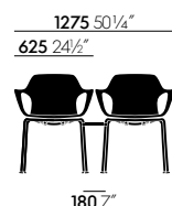
HAL Armchair with linking connectors
